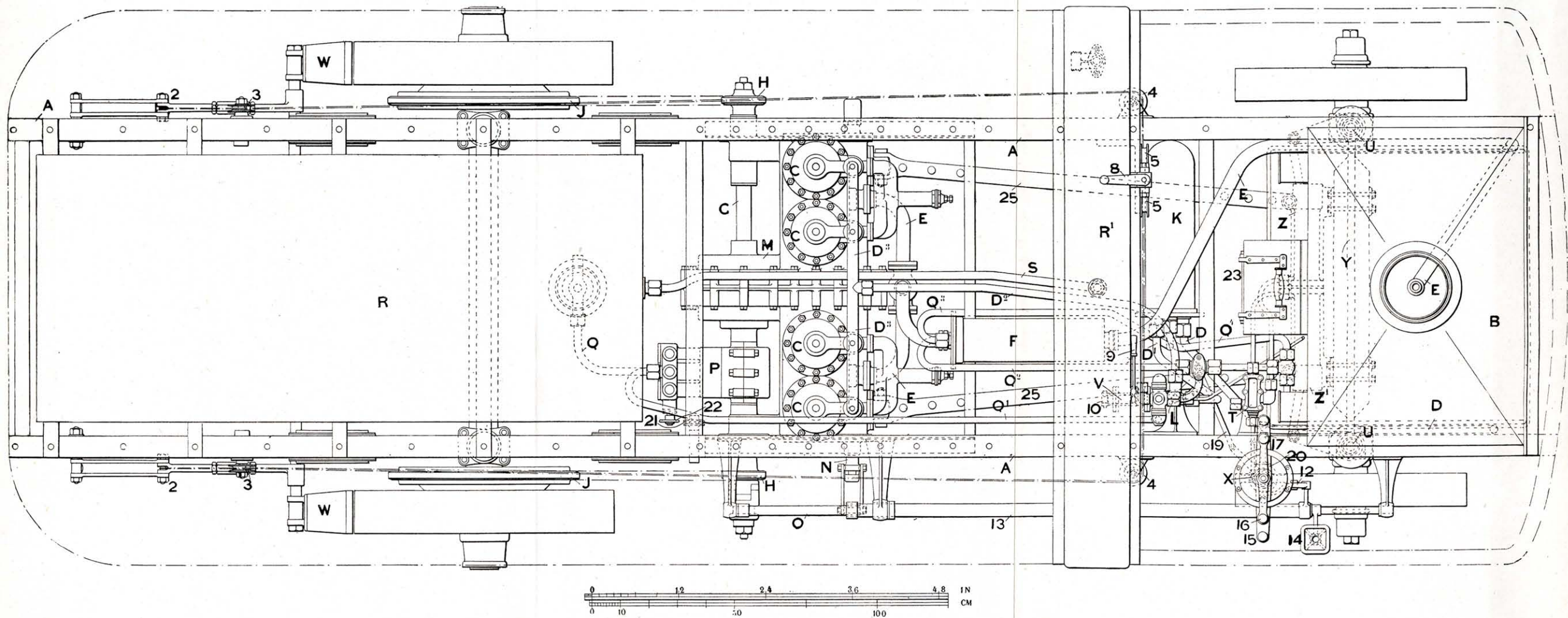
FIG. 336.—PLAN OF SIMPSON AND BIBBY'S 7-TON STEAM WAGON WITH 4-CYLINDER ENGINE.
