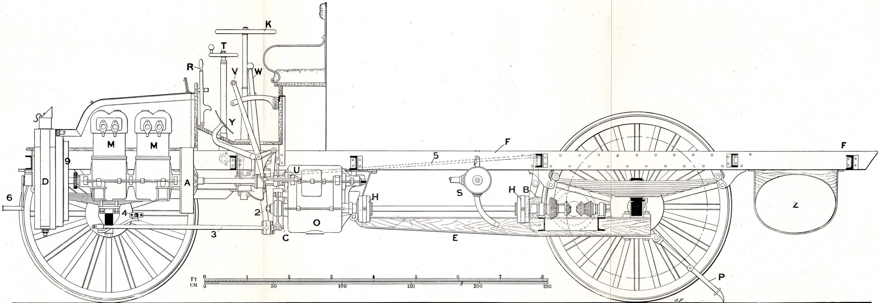
FIG. 373.—MILNES-DAIMLER 5-6-TON PETROL MOTOR LORRY. 16 HP.
