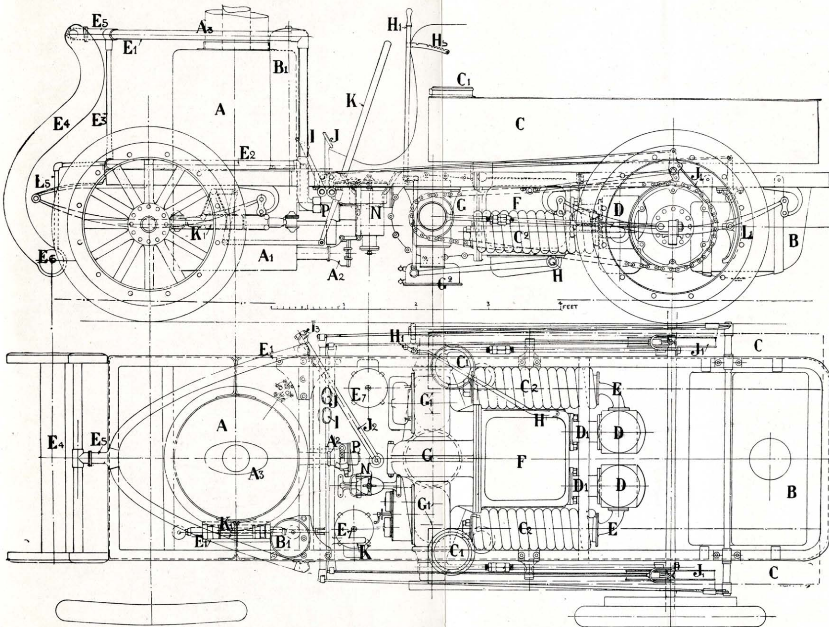
FIGS. 401 and 402.—CLARKSON STEAM CAR: ELEVATION AND PLAN WITH BODY REMOVED.
