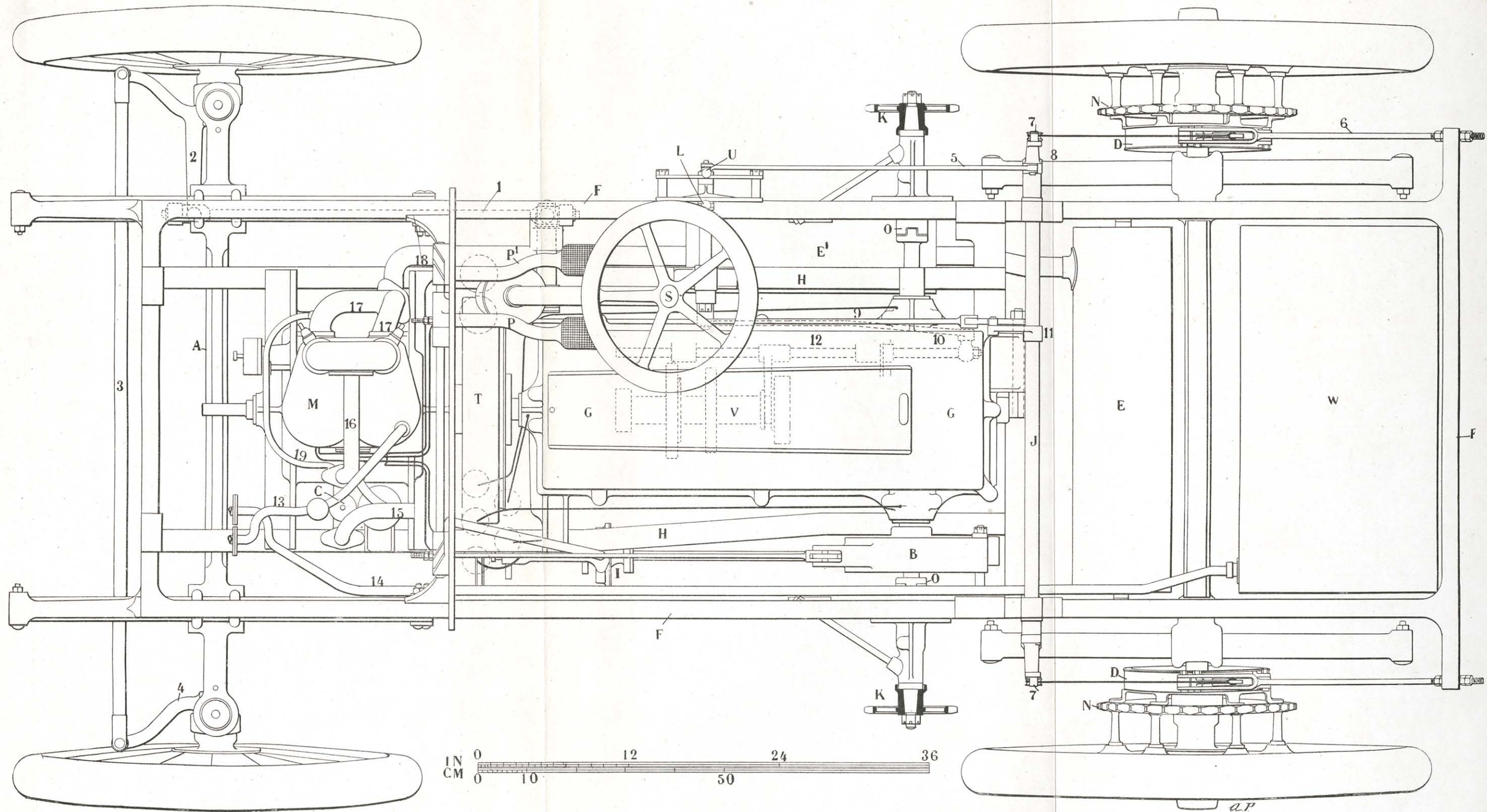
FIG. 252.—NAPIER TOURING CAR, 9 HP. 1902: PLAN.
