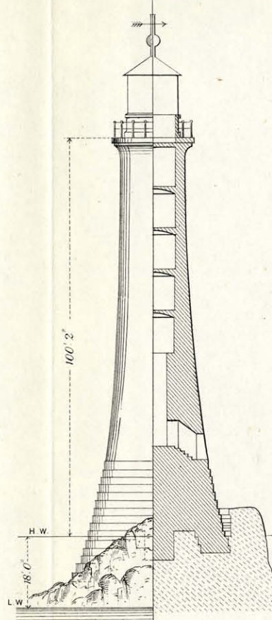
Fig. 7. BISHOPS ROCK.
