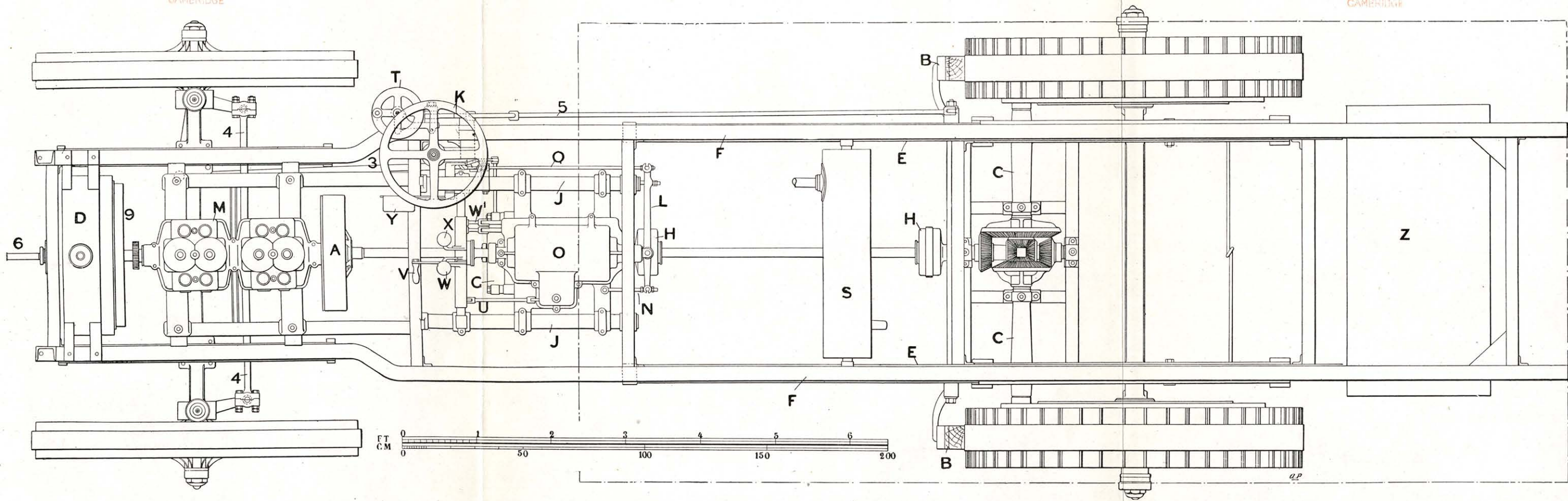
FIG. 374.—MILNES-DAIMLER 5-6-TON PETROL MOTOR LORRY. 16 HP. PLAN.
