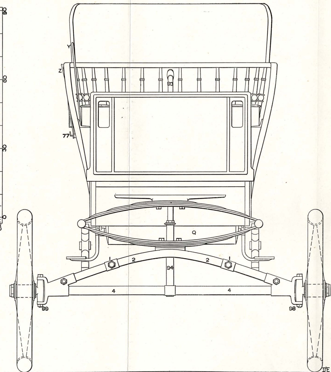
FIG. 345.—THE STANLEY CAR: FRONT ELEVATION.
