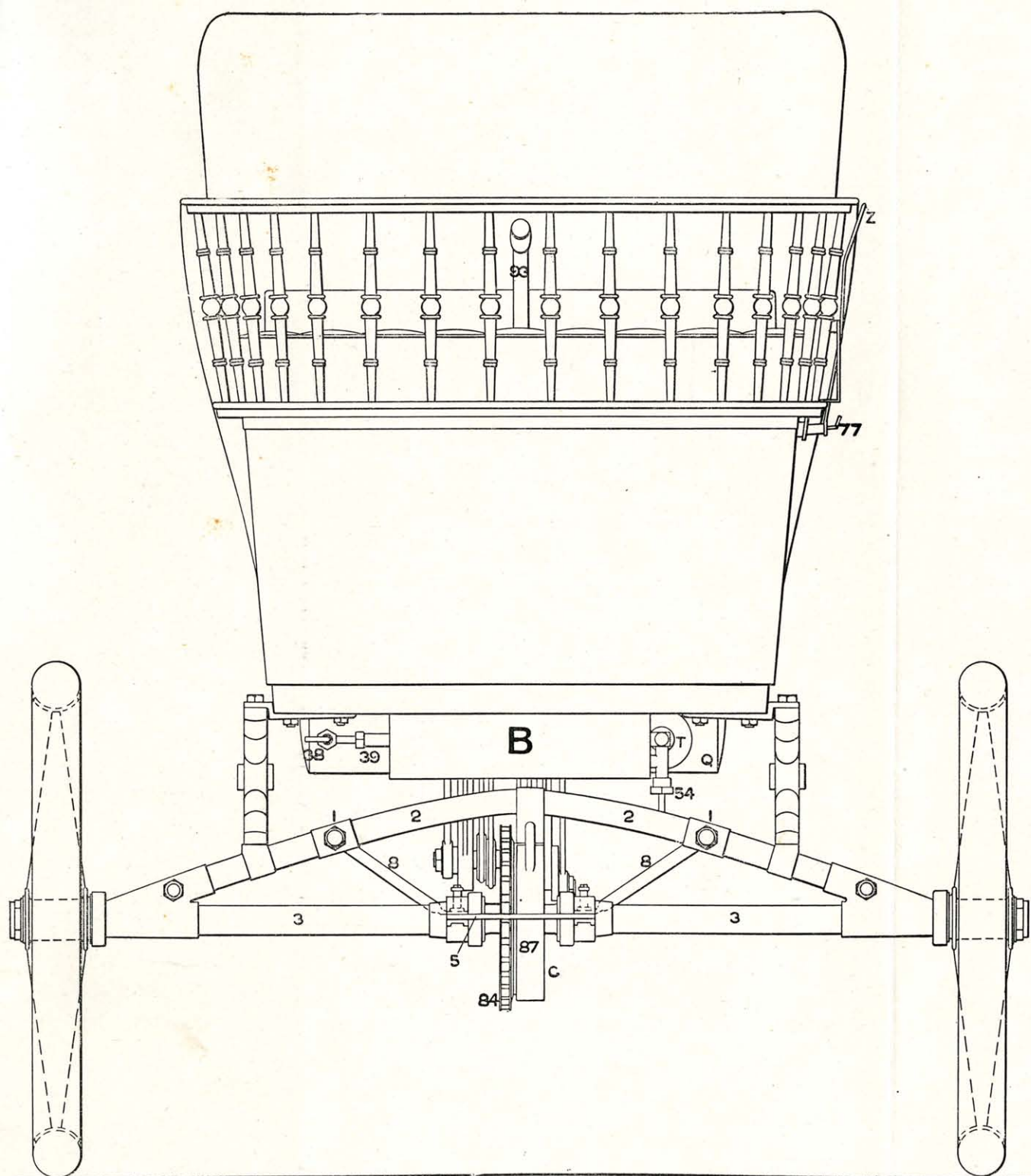
FIG. 344.—THE STANLEY LIGHT STEAM CAR: BACK ELEVATION.
