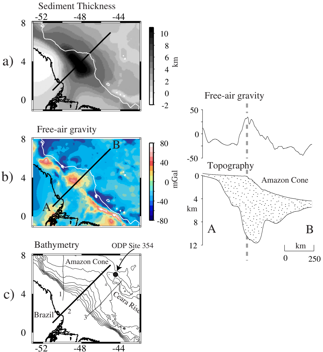
Fig. 4.40. Sediment thickness, gravity anomaly and bathymetry at the Amazon Cone, north-east Brazilian continental margin. (a) Sediment thickness based on Kumar et al. (1979). (b) Satellite-derived free-air gravity anomaly. (c) Bathymetry.
