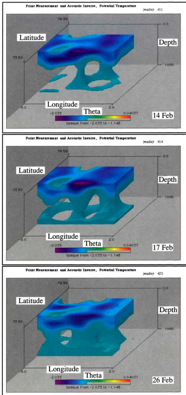
Fig. E.2. Formation and evolution of convective chimney structures in the Greenland Sea. Water with potential temperature less than -1.14^{\circ}\text{C} is contained within the colored blobs. In the period from 14 to 26 February 1989, the subsurface maximum virtually disappears. (From Morawitz et al. , 1994, with permission.)
