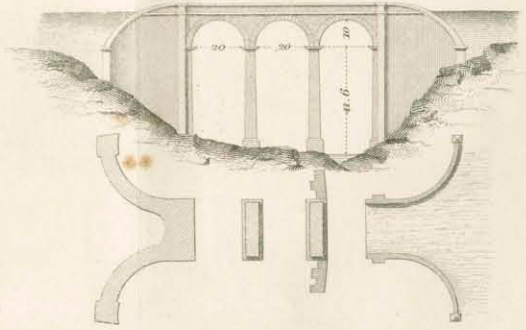
Fig. 7. Fidler Burn Bridge.
