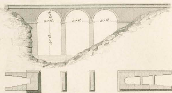
Fig. 6. Birkwood Burn Bridge.
